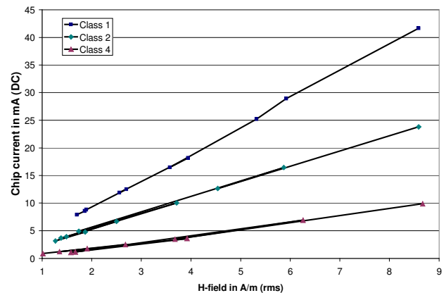
Figure 6. Available Chip current in mA (DC) measured for different Antenna Classes in Operating Volume.
