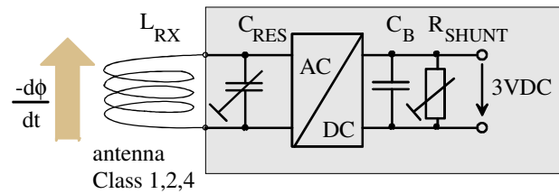
Figure 5. Reference PICC principle schematics.
