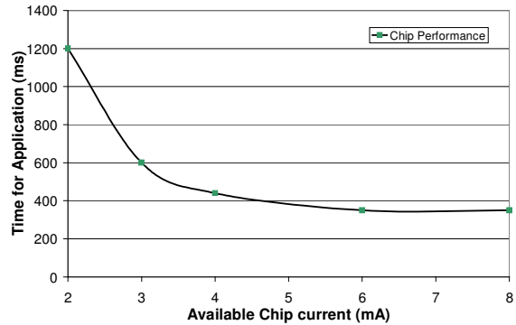
Figure 11. Application time depending on chip current.
